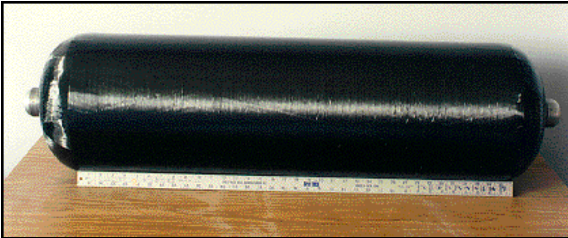
Figure 6. Scorpius test tanks. The tanks have a metallic liner and will be tested shortly for performance in holding LOX and kerosene.
